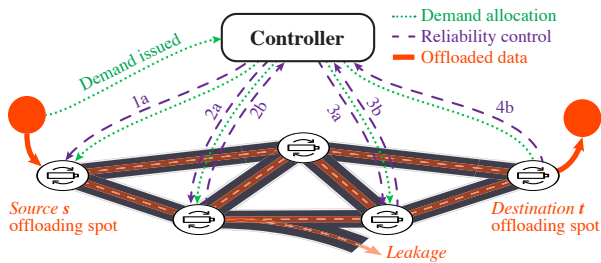
Fig. 5: Controller-to-offloading spot communication for the hop-by-hop (dashed arrows 1a-3a and 2b-4b) and end-to-end (dashed arrows 1a, 4b) retransmission strategies.
