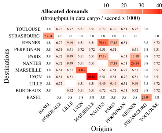
Fig. 14: Traffic matrix of the cities depicted in Figure 13 with the throughput of allocated demands expressed in terms of data cargo per second \times 1000.
